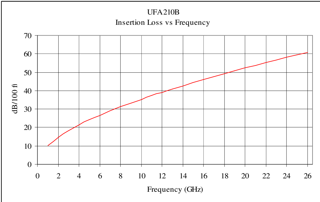
Fig. 4 UFA210B Maximum Insertion Loss
